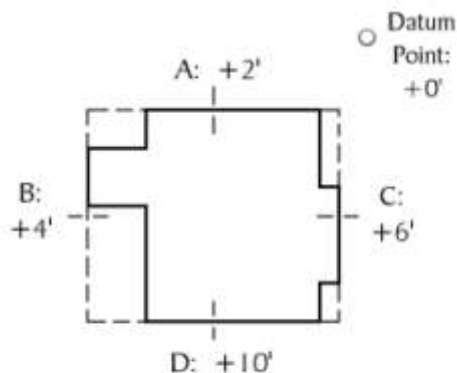
Diagram A How to Measure Building Height
